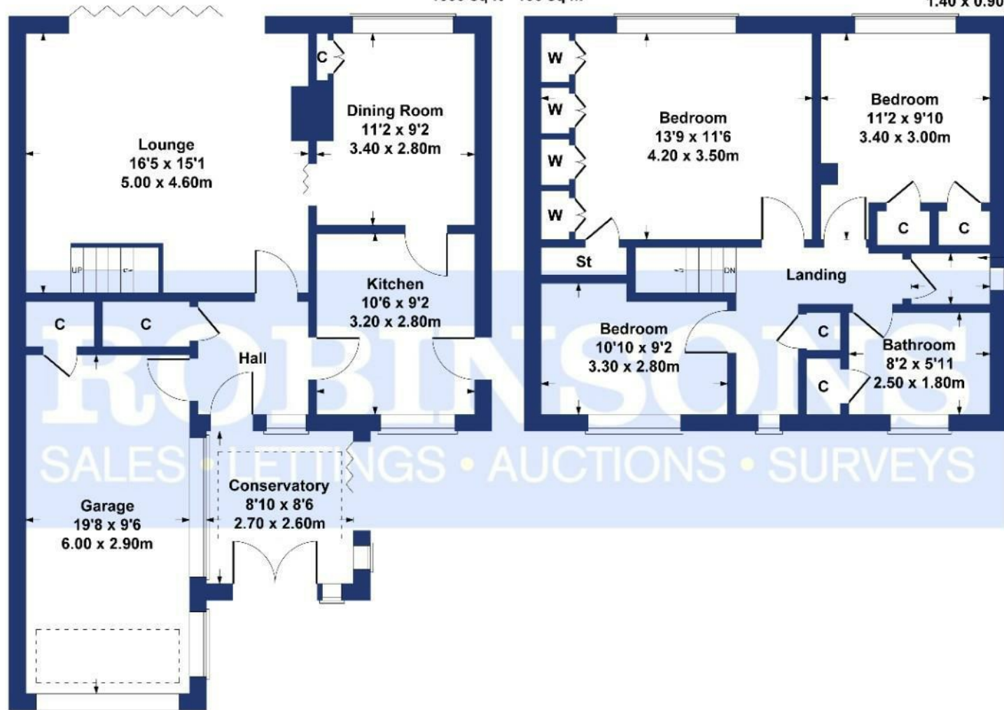
GROUND FLOOR
